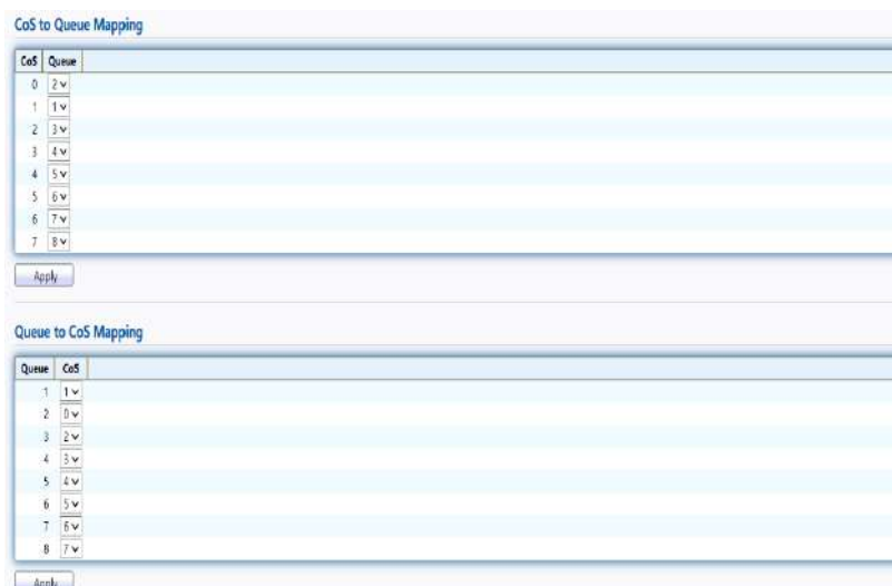
Figure 179 - QoS > General > Cos Mapping
