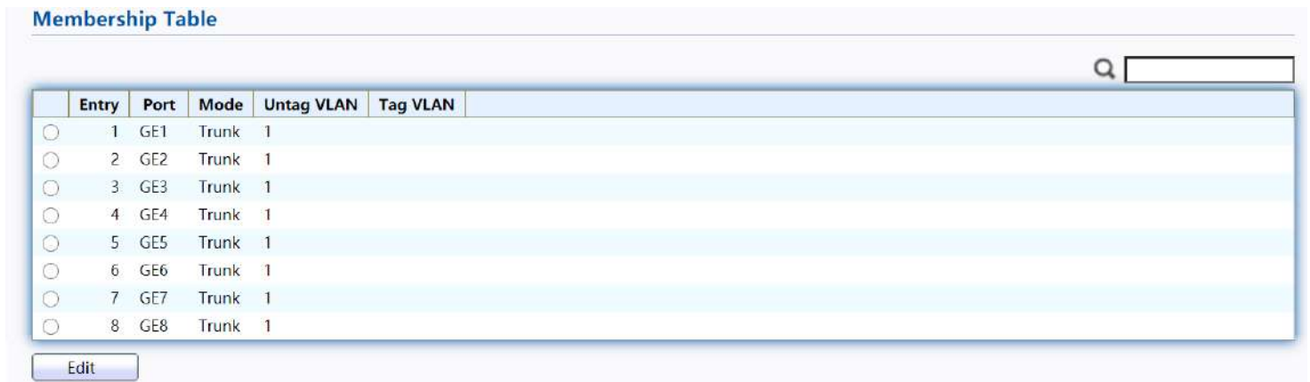
Figure 30 - VLAN > VLAN > Membership
